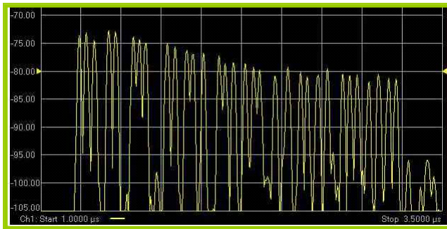
Figure 6: Experimental measurement of a 64 bit EPC Global SAW Tag. The tag is implemented using a 128 bit tag platform and includes encoding for anti-collision, multi-level error detection and other features. Insertion loss for the back end pulses is -53 dB. Vertical scale: 5 dB / division. Horizontal scale 0.25 microseconds per division from 1 to 3.5 microseconds.
