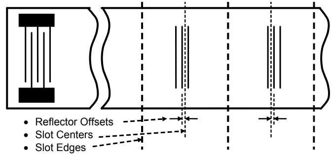
Figure 4: Two slots of an un-encoded Global SAW Tag with 3 open-circuit reflectors per slot and showing the locations of slot edges, slot centers, and reflector offsets as needed to produce desired slot phase shifts.
