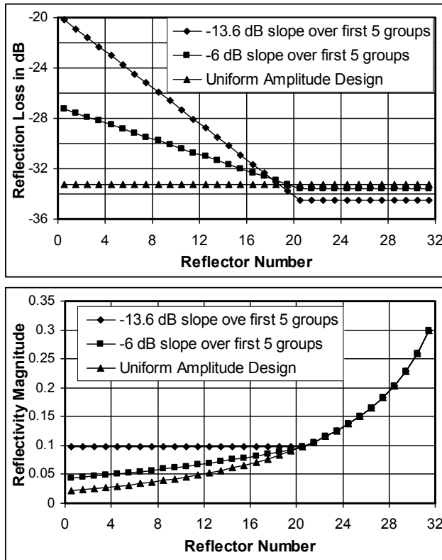
Figure 3: Three single track design variations for a 128 bit Global SAW Tag platform using Equation 3. Top shows reflection loss not including losses from the transducer and pedestal delay. The bottom figure shows individual reflector strengths. Average pulse spacings were assumed for these calculations.
