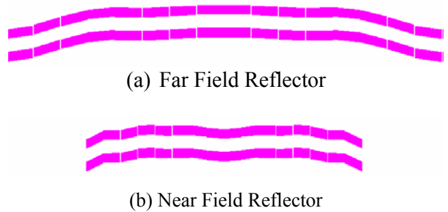
Figure 5: Two diffraction-compensated reflector layouts for a 94 wavelength beamwidth tag device. The x and y axes are distorted by 22:1 for purposes of clarity.
