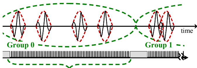
Figure 1: Each 16 bit data group has pulses placed in 4 of 75 slots time of \sim 3.05 nsec. width, with -64^\circ phase shift per slot. A minimum pulse separation of 12 time slots is enforced to allow detection of individual pulses under the Nyquist criteria. Also, 11 unoccupied slots exist between groups for this same purpose.
